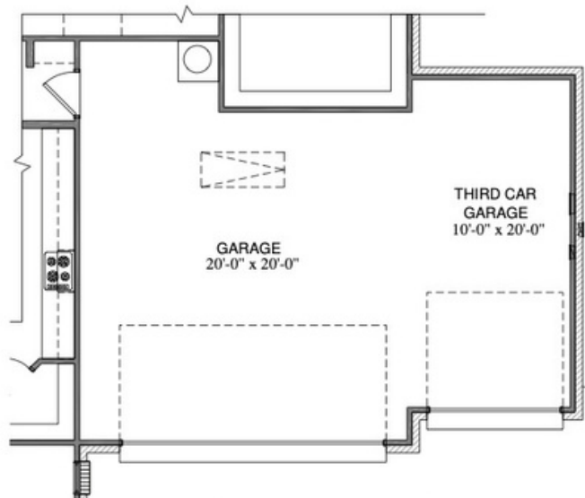
OPT. THIRD CAR GARAGE *AVAILABLE ON INTERIOR LOTS LARGER THAN 60' AND CORNER LOTS LARGER THAN 75'
