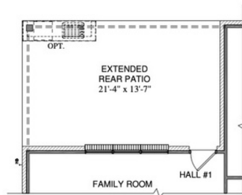
OPT. EXTENDED REAR PATIO
