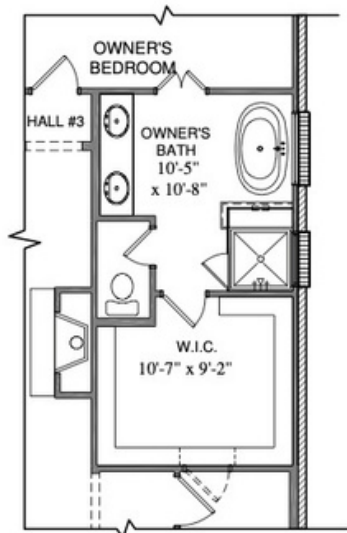
OPT. LUXURY OWNER'S BATH W/ FREE-STANDING TUB
