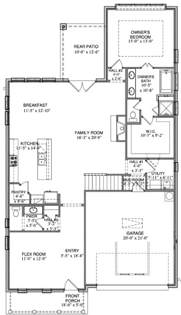
FIRST FLOOR
