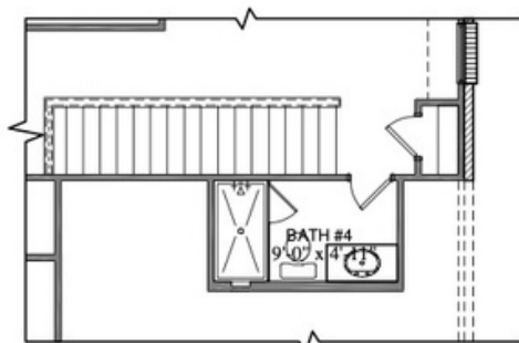
OPT. BATH #4 SHOWER
