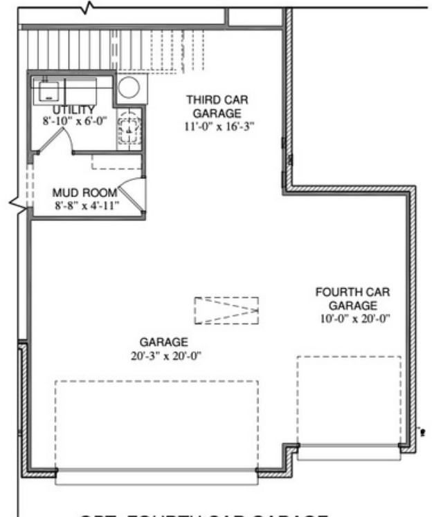
OPT. FOURTH CAR GARAGE *AVAILABLE ON INTERIOR LOTS LARGER THAN 60' AND CORNER LOTS LARGER THAN 75'
