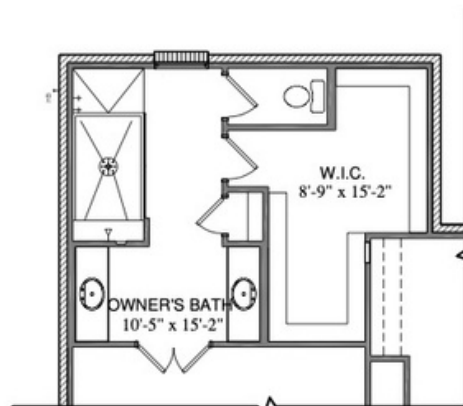
OPT. OWNER'S BATH SHOWER
