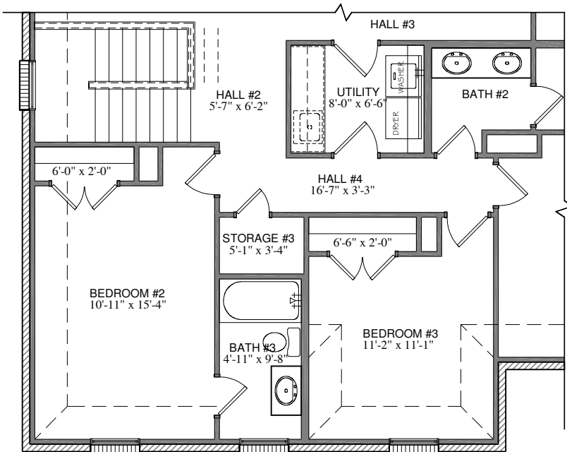
OPT. BATH #3- ELEVATION "C"
