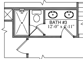
OPT. BATH #3 SHOWER
