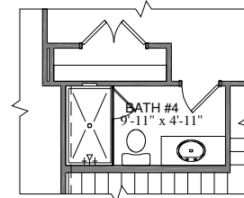
OPT. BATH #4 SHOWER
