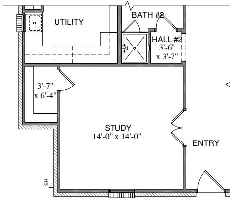
OPT. STUDY - ELEV "A, C & D"
