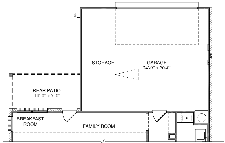
OPT. GARAGE STORAGE W/ OPT. REAR PATIO
