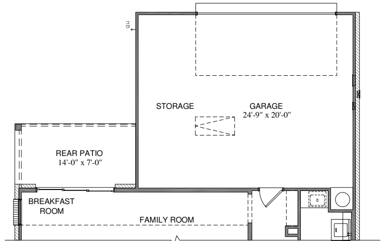
OPT. GARAGE STORAGE W/ OPT. REAR PATIO W/ OPT. SLIDING DOOR UNIT
