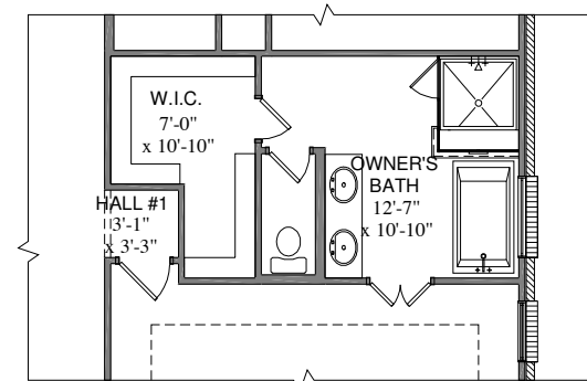
OPT. LUXURY OWNER'S BATH
