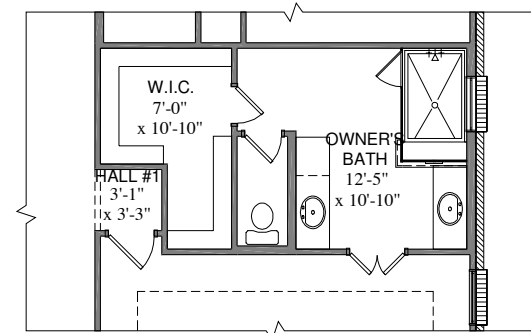
OPT. OWNER'S BATH SHOWER
