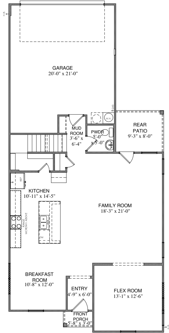
FIRST FLOOR
