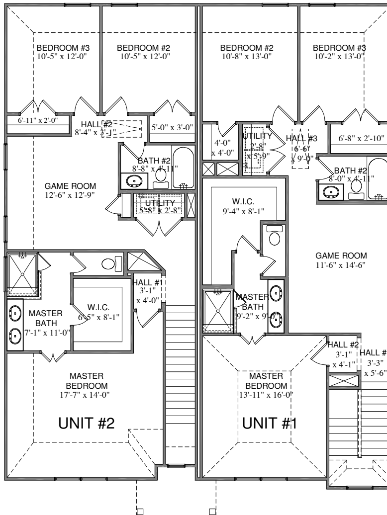
SECOND FLOOR PLAN ELEVATION "A"
