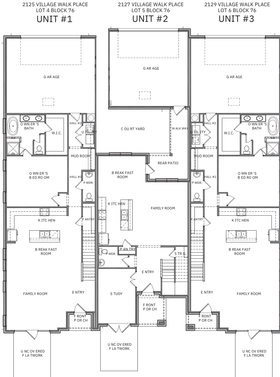
FIRST FLOOR PLAN ELEVATION "A"
