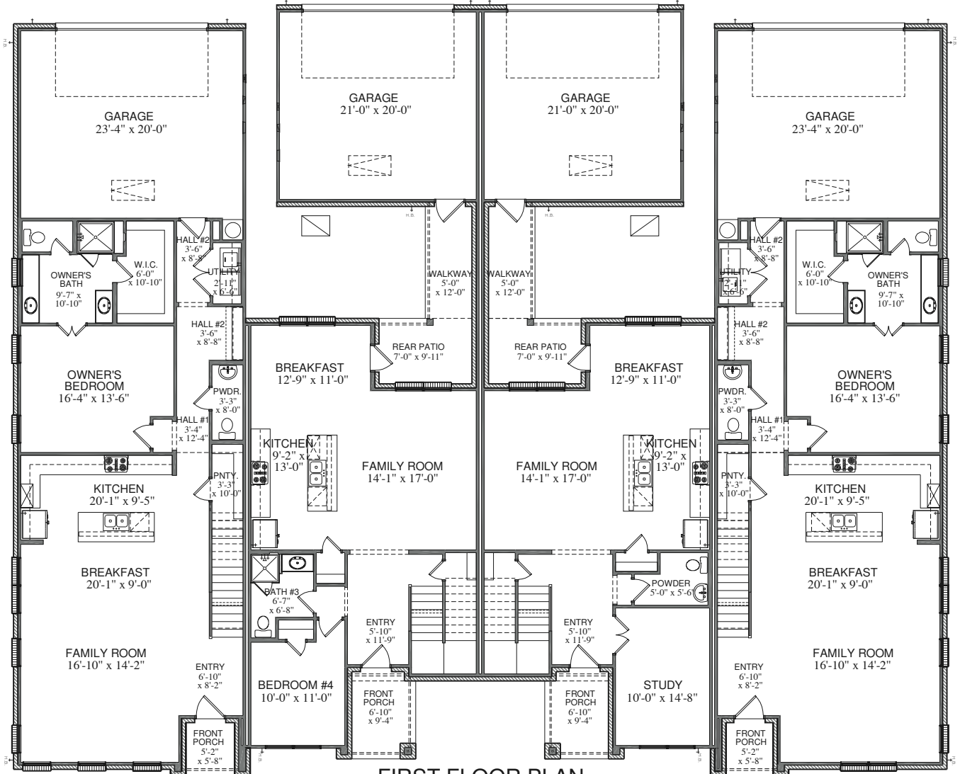
FIRST FLOOR PLAN SQUARE FOOTAGE TOTALS
