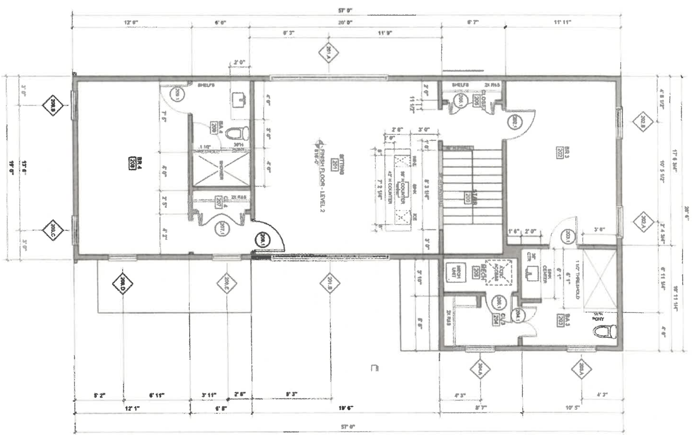
FLOOR PLAN - LEVEL TWO
