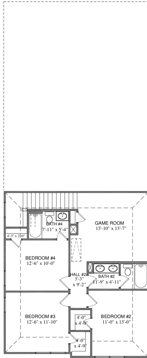
SECOND FLOOR
