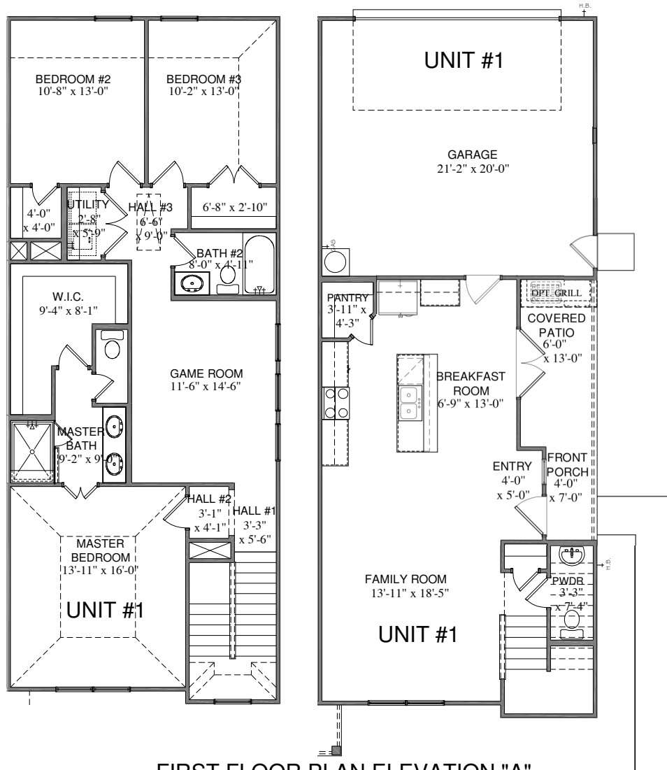
FIRST FLOOR PLAN ELEVATION "A" SQUARE FOOTAGE TOTALS UNIT #1
