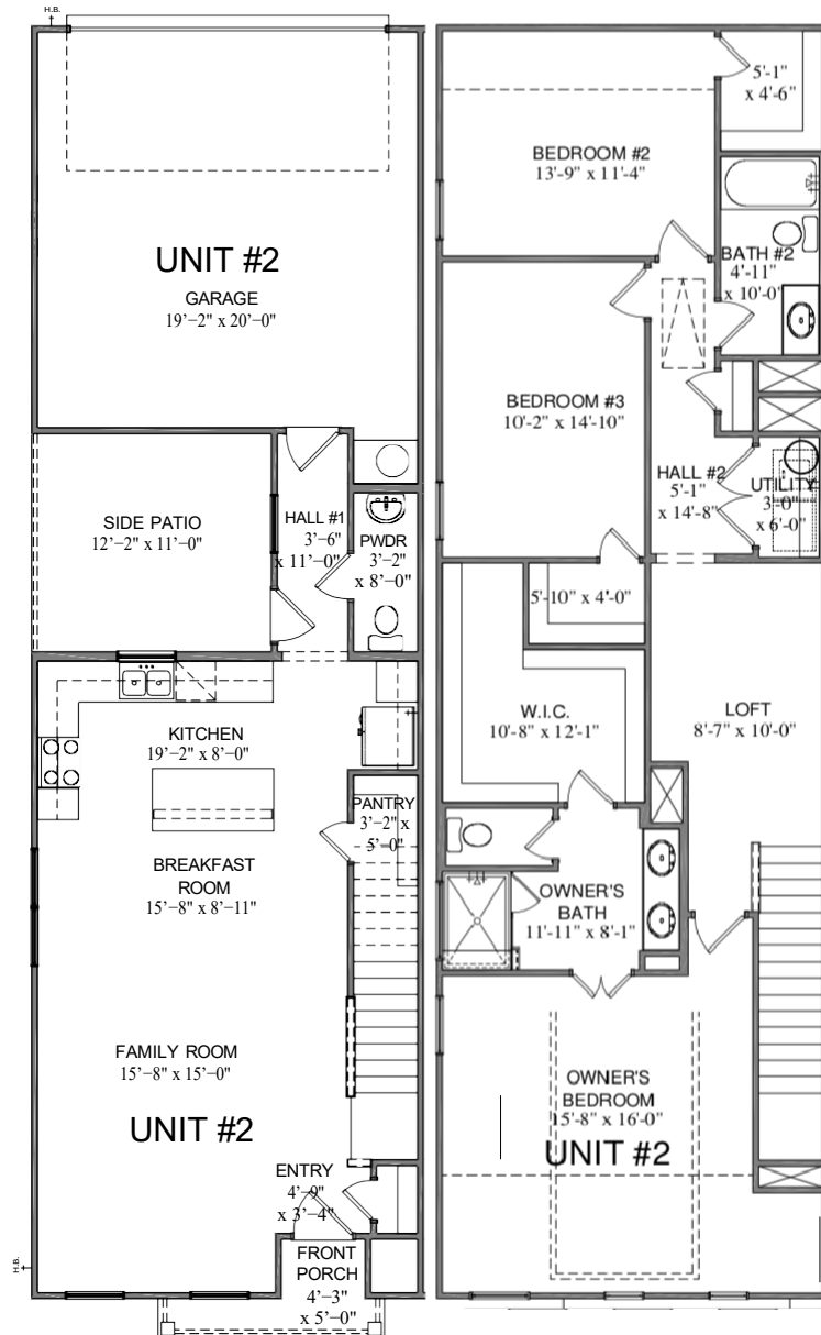
FIRST FLOOR PLAN ELEVATION "A" SQUARE FOOTAGE TOTALS
