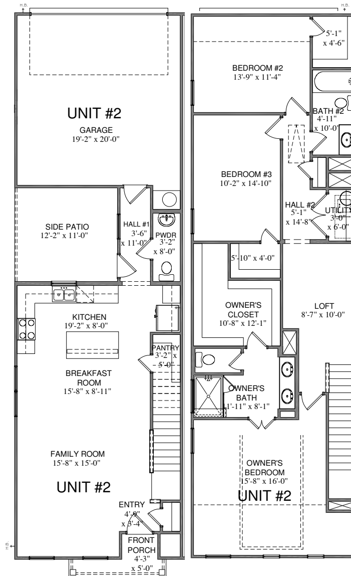
FIRST FLOOR PLAN ELEVATION "B" SQUARE FOOTAGE TOTALS
