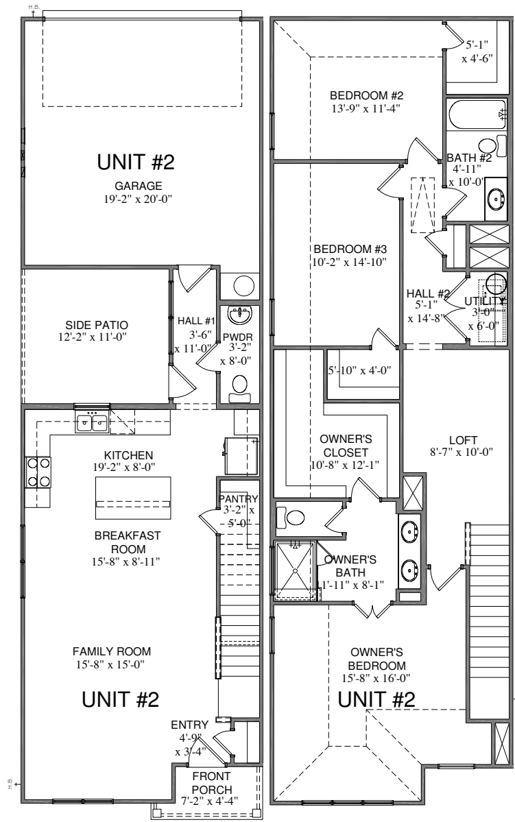
FIRST FLOOR PLAN ELEVATION "A" SQUARE FOOTAGE TOTALS
