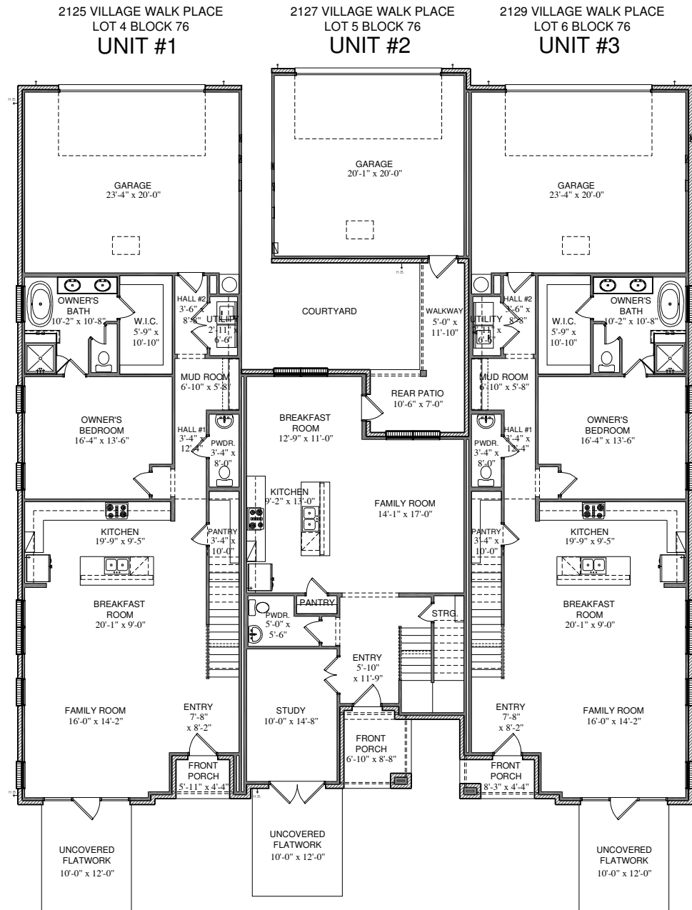
FIRST FLOOR PLAN ELEVATION "A" SQUARE FOOTAGE TOTALS
