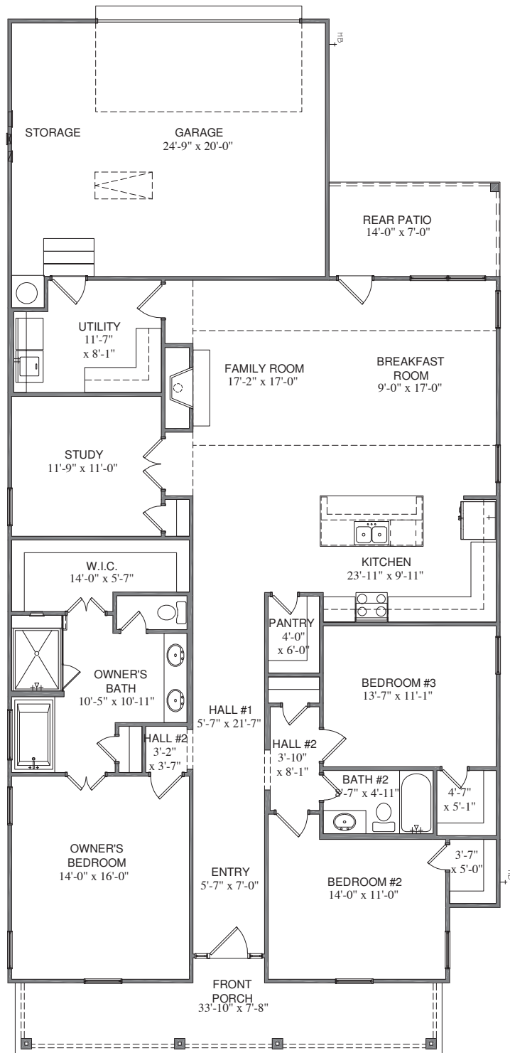
FLOOR PLAN
